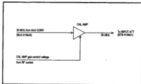
Figure 3-16 CAL Amplifier
