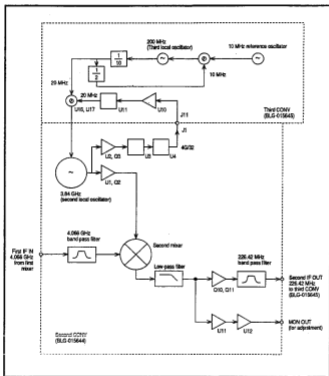
Figure 3-5 Second Mixer/Second Local Oscillator
