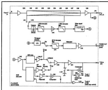
Figure 3-9 LOG/QP
