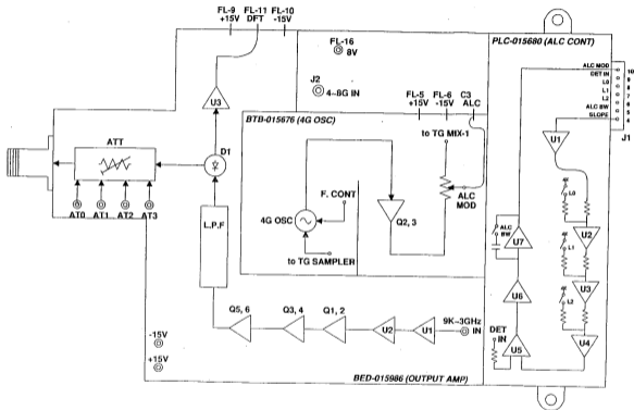
CIRCUIT LAYOUT TG BLOCK 2 WBL-3361TG BED-015986 BLC-015680 BTB-015676
