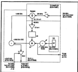
Figure 3-20 4GHz Oscillator
