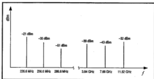
Figure 3-6 Spectrum Distribution at the MON OUT Terminal
