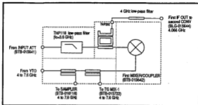
Figure 3-4 First Mixer/Coupler
