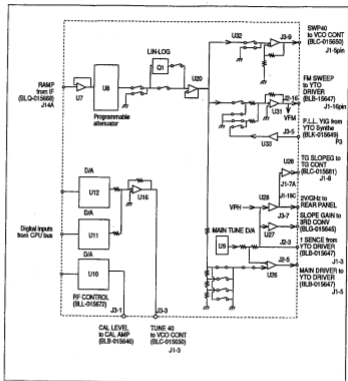
Figure 3-14 RF Control
