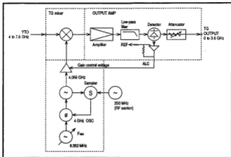
Figure 3-17 Tracking Generator Block Diagram
