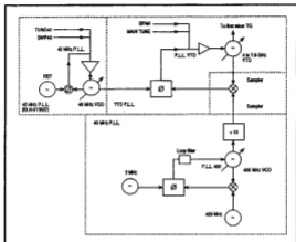
Figure 3-11 First Local Oscillator
