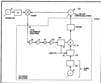
Figure 3-13 YTO P.L.L.
