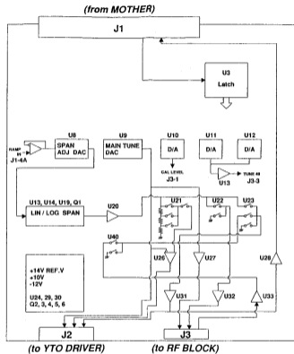
CIRCUIT LAYOUT RF CONTROL BLL-015672
