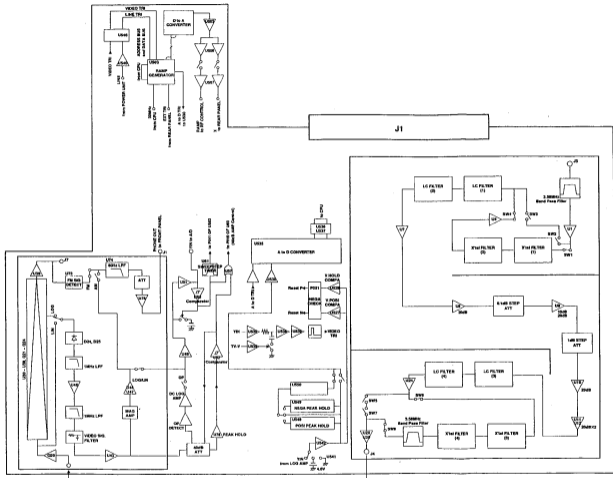
CIRCUIT LAYOUT IF SECTION BLQ-015668
