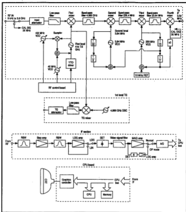
Figure 3-2 R3261/3361 Block Diagram
