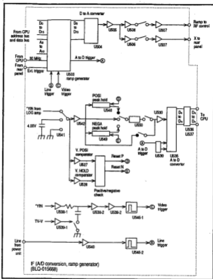
Figure 3-10 A/D Conversion and Ramp Generator
