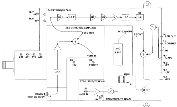
CIRCUIT LAYOUT TG BLOCK 1 WBL-3361TG BLB-015987 BLD-015988 BTB-015722 BTB-015723
