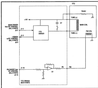
Figure 3-15 YTO Driver
