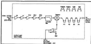
Figure 3-18 Output Amplifier
