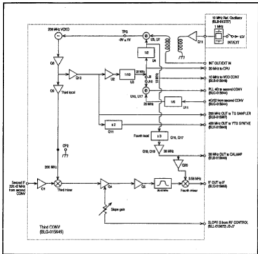
Figure 3-7 Third and Fourth Mixers and Local Oscillators
