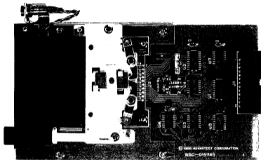
PARTS LOCATION IC CARD BGC-015745
