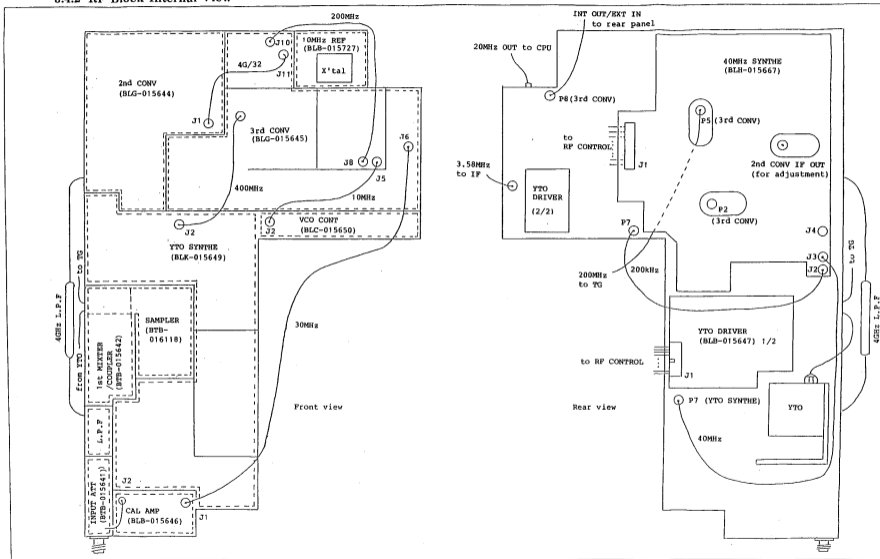
Figure 3-25 RF Block Internal View
