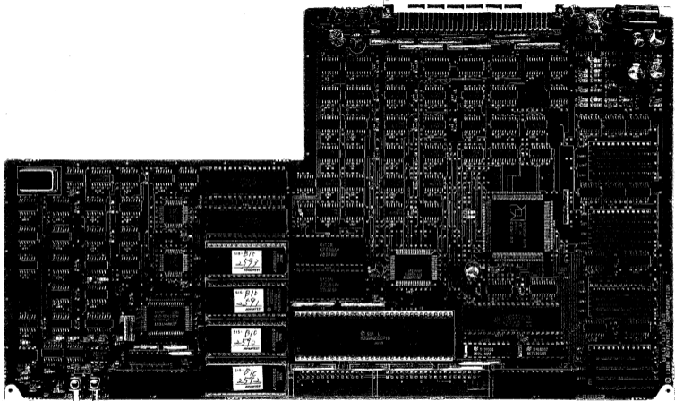
PARTS LOCATION CPU BLQ-015669
